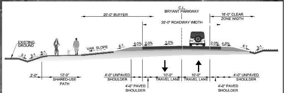
BRYANT PARKWAY: TYPICAL SECTION
